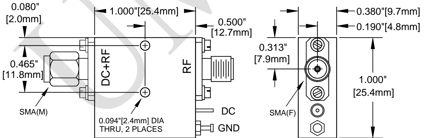
Fig. 1-B (Option "B2" <> BT-XXB2-LS)
