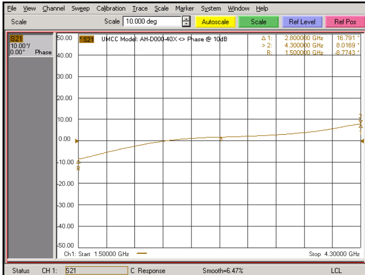
Phase Shift @ 10dB Attn.
