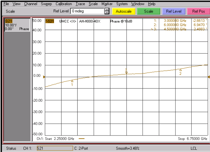
Phase Shift @ 10dB Attn.
