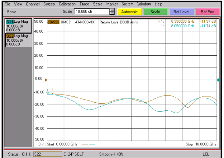
Input / Output Return Loss @ 80dB Attn
