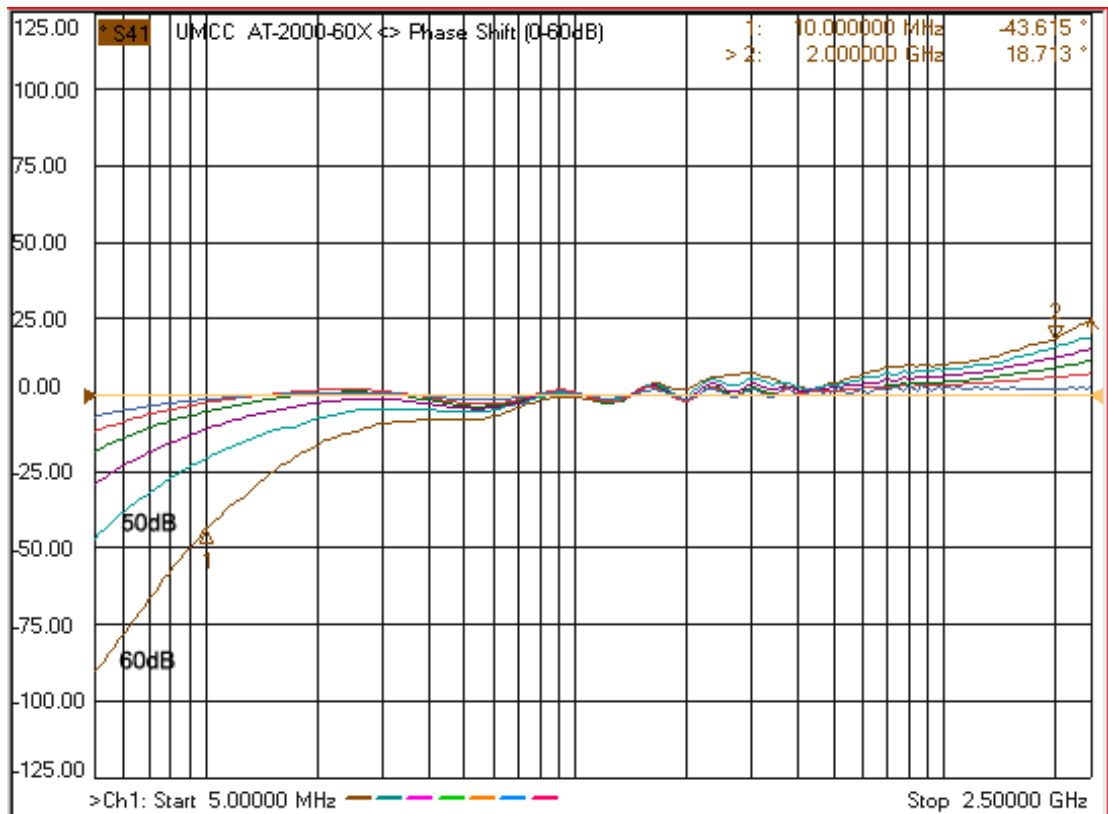
- Phase Variation
