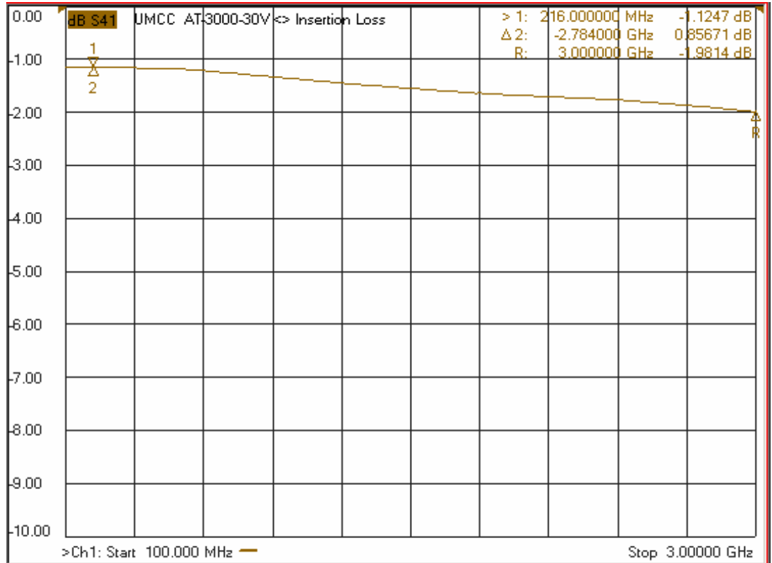
- Insertion Loss
