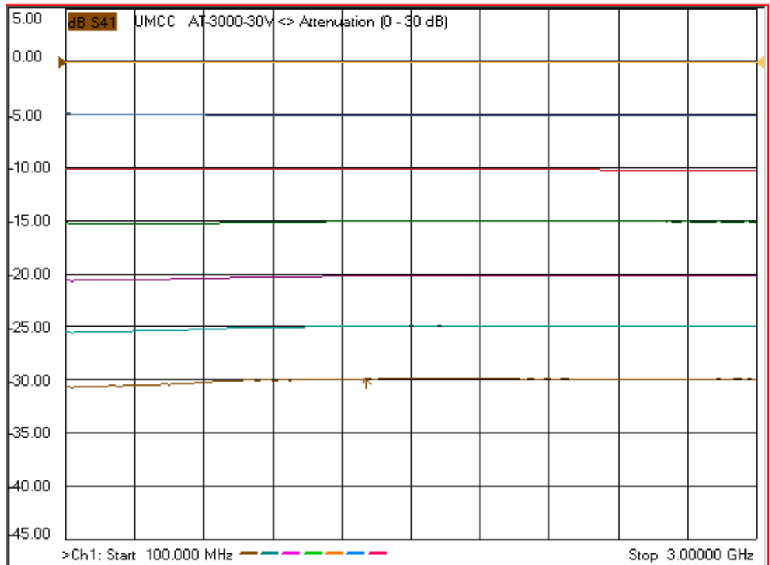
- Attenuation Range
