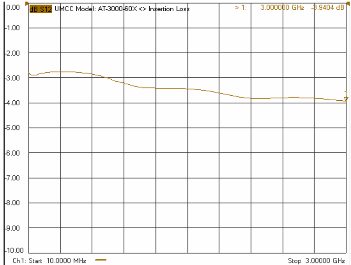
- Insertion Loss
