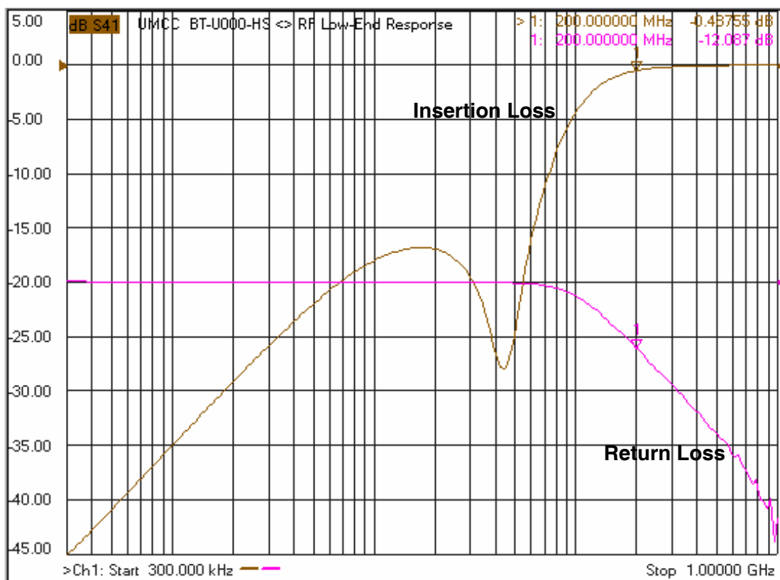
- Out-Band Low-End Freq. Response
