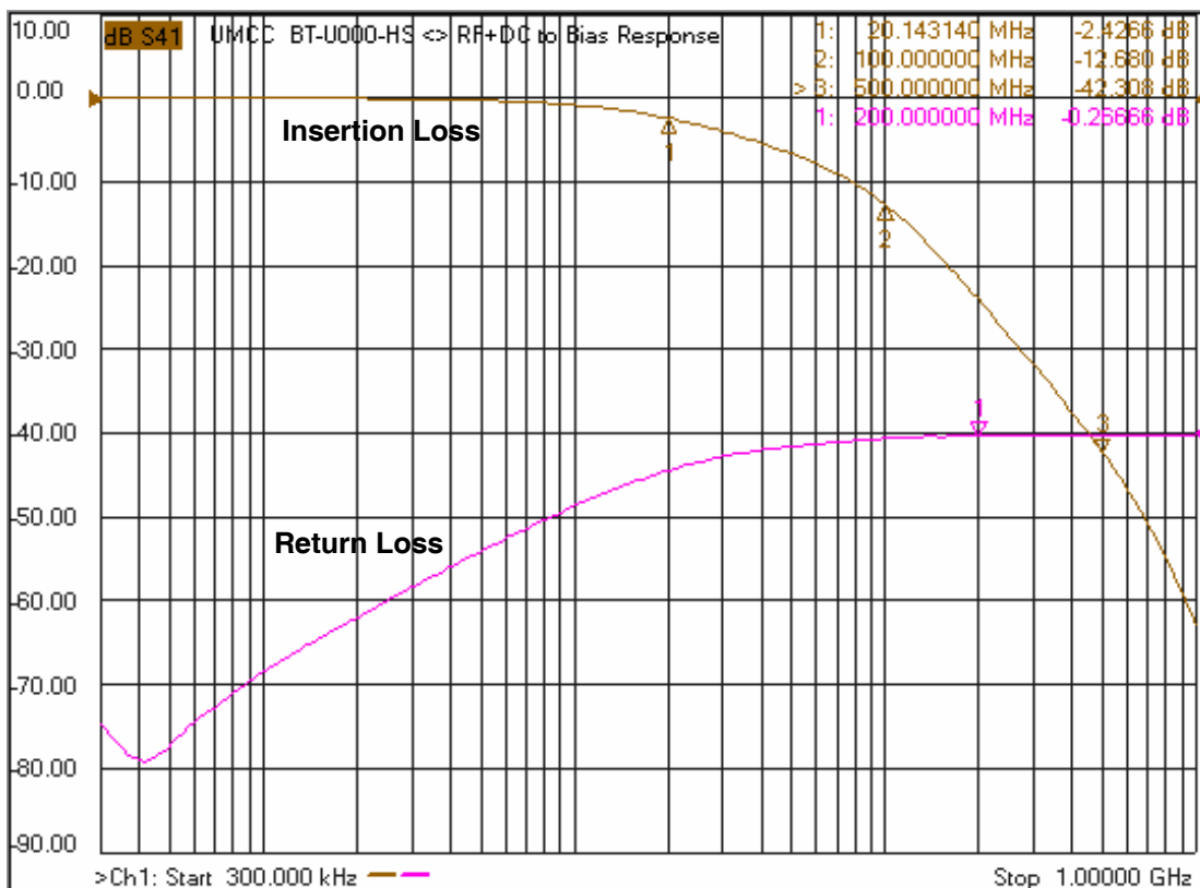
- Bias Freq. Response (Bias to RF+DC)
