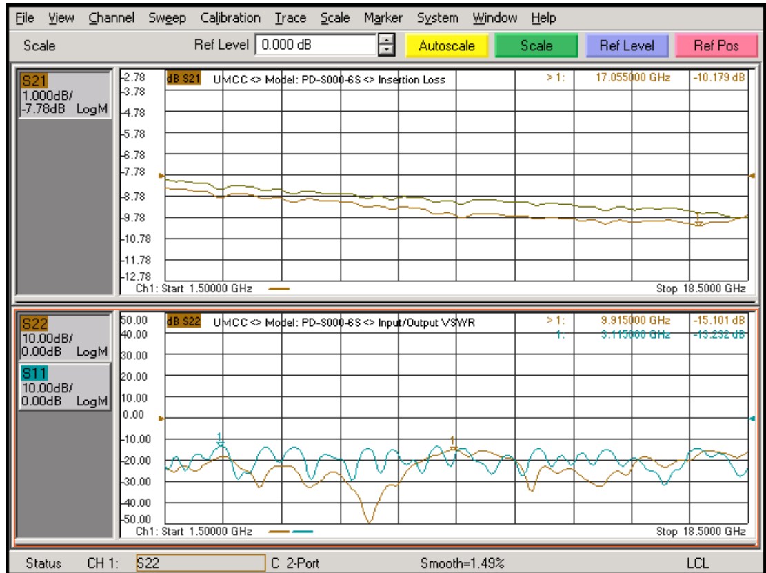
-Insertion Loss
