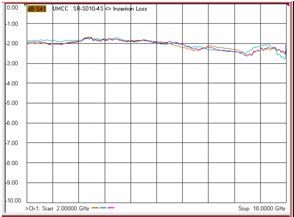
-Insertion Loss
