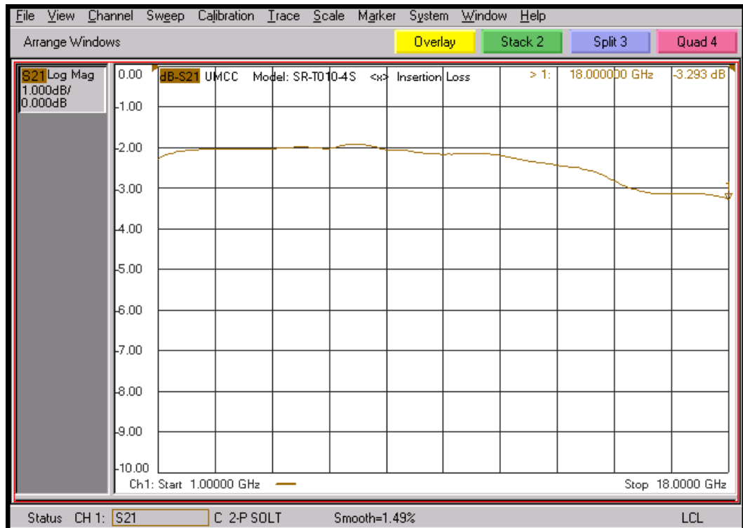
-Insertion Loss
